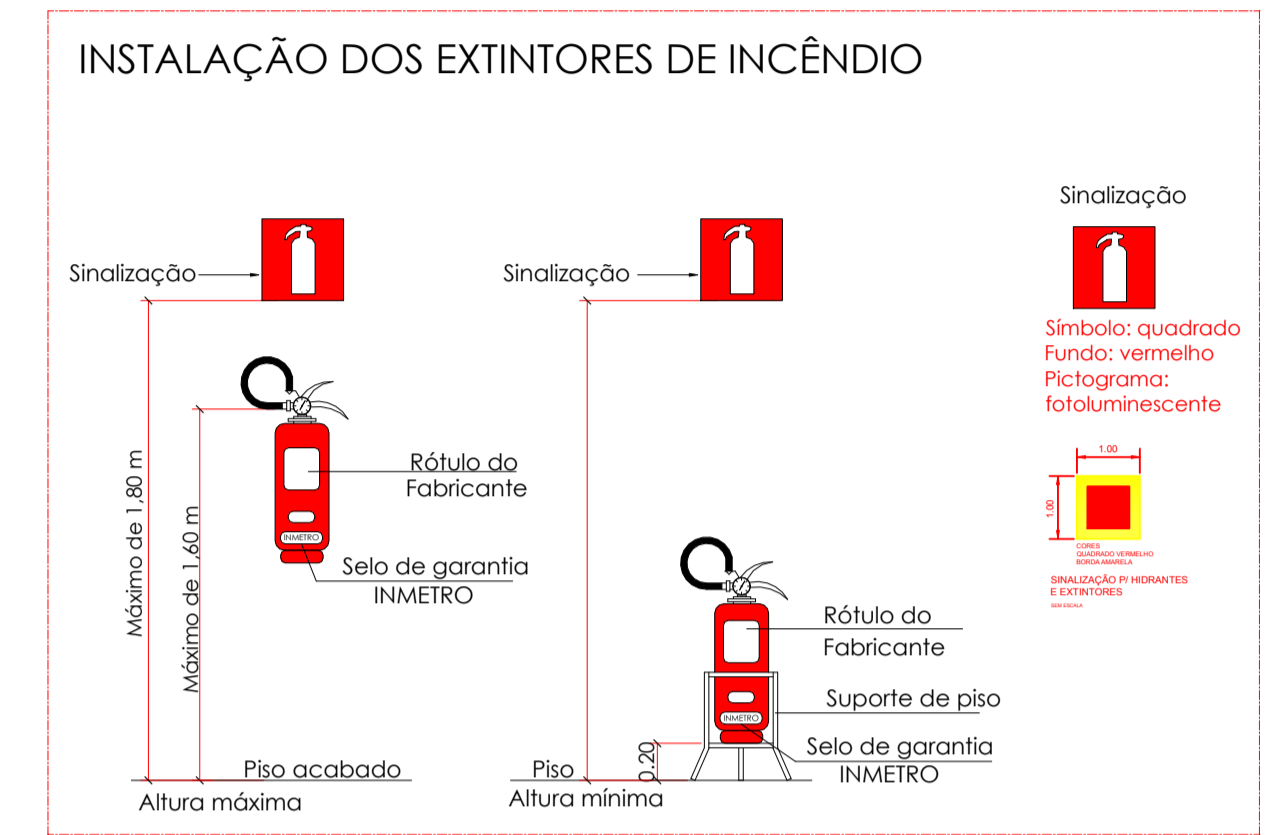
DETAILHE 02 S/ESCALA
