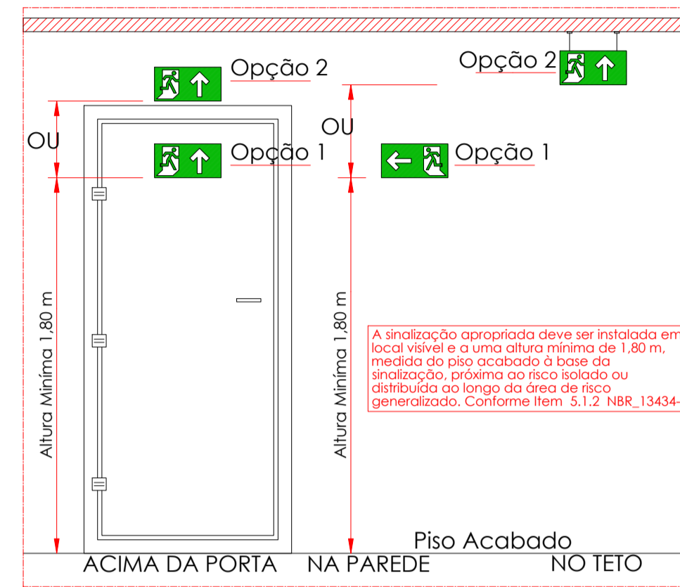
DETAILHE 01 S/ESCALA
